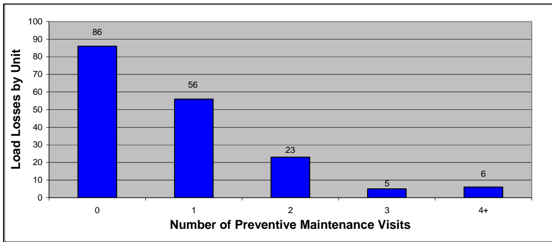
Chart 1: Eaton UPS load losses by preventive maintenance visits delivered in prior year.
